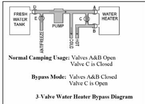
Factory installed 3-valve water heater bypass
